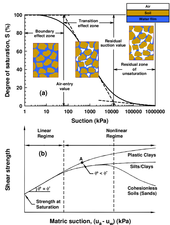
Figure 1. (a) SWCC illustrating zones of desaturation; (b) The relationship between the SWCC with shear strength of unsaturated soils (Vanapalli, 2009)
